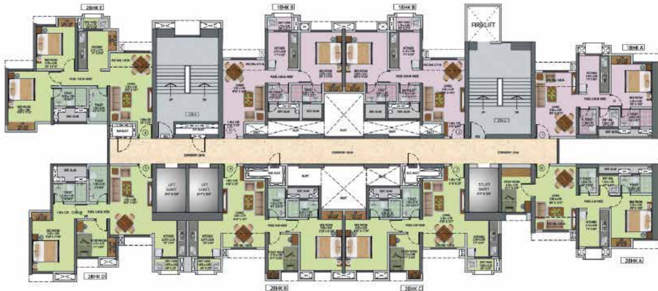
TYPICAL FLOOR PLAN (WITHOUT PATIO) FLOOR - 4,6,8,10,12,14,16,18,20,22,24,26,28,30,32,34,36,38,40
